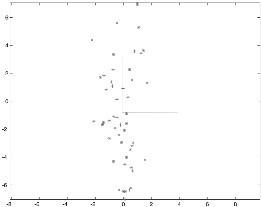
FIGURE 16.11: A dataset that is well represented by a principal component analysis. The axes represent the directions obtained using PCA; the vertical axis is the first principal component, and is the direction in which the variance is highest.
