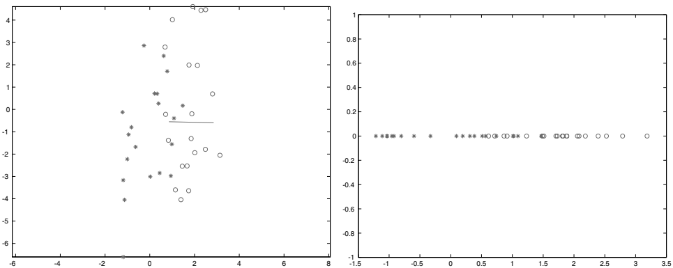
FIGURE 16.14: Canonical variates use the class of each data item as well as the features in estimating a good set of linear features. In particular, the approach constructs axes that separate different classes as well as possible. The dataset used in Figure 16.13 is shown on the left , with the axis given by the first canonical variate overlaid. On the bottom right , we show the projection onto that axis, where the classes are rather well separated.
