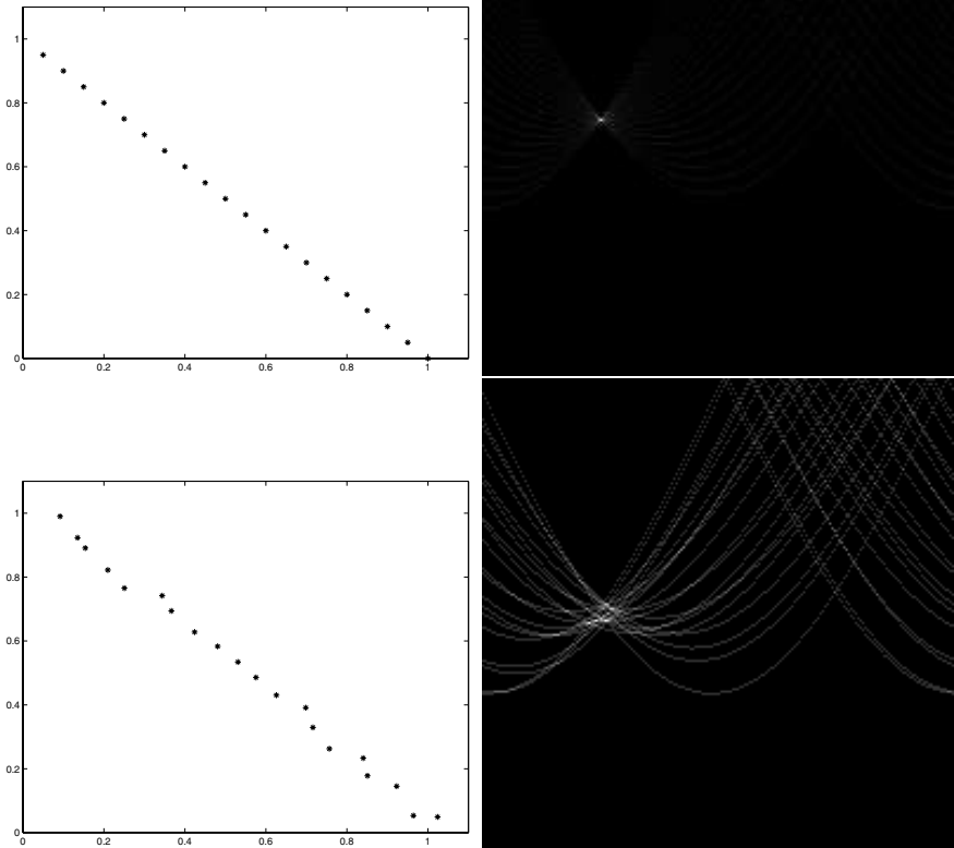
FIGURE 10.1: The Hough transform maps each point like token to a curve of possible lines (or other parametric curves) through that point. These figures illustrate the Hough transform for lines. The left-hand column shows points, and the right-hand column shows the corresponding accumulator arrays (the number of votes is indicated by the gray level, with a large number of votes being indicated by bright points). The top row shows what happens using a set of 20 points drawn from a line. On the top right , the accumulator array for the Hough transform of these points. Corresponding to each point is a curve of votes in the accumulator array; the largest set of votes is 20 (which corresponds to the brightest point). The horizontal variable in the accumulator array is \theta , and the vertical variable is r ; there are 200 steps in each direction, and r lies in the range [0, 1.55] . On the bottom , these points have been offset by a random vector, each element of which is uniform in the range [0, 0.05] . Note that this offsets the curves in the accumulator array shown next to the points and the maximum vote is now 6 (which corresponds to the brightest value in this image; this value would be difficult to see on the same scale as the top image).
