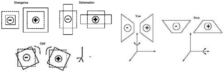
FIGURE 10.14: Typical flows generated by the model (u(x), v(x))^T = (\theta_1 + \theta_2 x + \theta_3 y + \theta_7 x^2 + \theta_8 xy, \theta_4 + \theta_5 x + \theta_6 y + \theta_9 xy + \theta_8 y^2) . Different values of the \theta_i give different flows, and the model can generate flows typical of a 2D figure moving in 3D. Divergence occurs when the image is scaled; for example, \theta = (0, 1, 0, 0, 0, 1, 0, 0) . Deformation occurs when one direction shrinks and another grows (for example, rotation about an axis parallel to the view plane in an orthographic camera); for example, \theta = (0, 1, 0, 0, 0, -1, 0, 0) . Curl can result from in plane rotation; for example, \theta = (0, 0, -1, 0, 1, 0, 0, 0) . Yaw models rotation about a vertical axis in a perspective camera; for example \theta = (0, 0, 0, 0, 0, 1, 0, 0) . Finally, pitch models rotation about a horizontal axis in a perspective camera; for example \theta = (0, 0, 0, 0, 0, 0, 1, 0) . This figure was originally published as Figure 2 of “Cardboard People: A Parameterized Model of Articulated Image Motion,” S. Ju, M. Black, and Y. Yacoob, IEEE Int. Conf. Face and Gesture , 1996 © IEEE, 1996.
