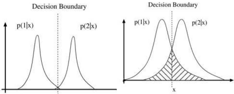
FIGURE 15.1: This figure shows typical elements of a two-class classification problem. We have plotted p(\text{class}|x) as a function of the feature x . Assuming that L(-1 \rightarrow 1) = L(1 \rightarrow -1) , we have marked the classifier boundaries. In this case, the Bayes risk is the sum of the amount of the posterior for class one in the class two region and the amount of the posterior for class two in the class one region (the hatched area in the figures). For the case on the left, the classes are well separated, which means that the Bayes risk is small; for the case on the right, the Bayes risk is rather large.
