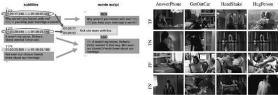
FIGURE 20.20: Laptev et al. (2008) learn discriminative models of actions by obtaining film scripts, where actions will be named, and then aligning subtitles in the film with the script ( left ) to get windows of film where an action is very likely to occur. With enough examples, they can learn a classifier despite the odd mislabeled example. This classifier can then be used to spot actions of considerable complexity. On the right , some examples of true positives (TP), true negatives (TN), false positives (FP), and false negatives (FN) for some complex actions detected with this method. This figure was originally published as Figure 10 of “Learning realistic human actions from movies,” by I. Laptev, M. Marszalek, C. Schmid, and B. Rozenfeld, Proc. IEEE CVPR 2008, © IEEE, 2008.
