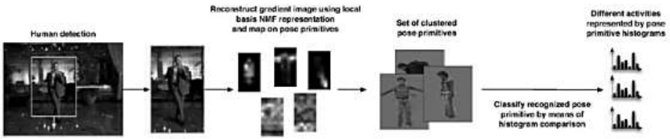
FIGURE 20.14: Many activities involve quite characteristic body poses. Thureau and Hlavac (2008) show that a simple and effective representation of composite activities can be built by finding these distinctive poses, then reporting a histogram. To provide some temporal information, the histogram contains n -grams of poses (i.e., sequences of n poses), rather than single poses. This representation performs well on established activity classification datasets, but also produces sensible reports when faced with novel activities. This figure was originally published as Figure 4 of “Action Recognition from a Distributed Representation of Pose and Appearance,” by C. Thureau and V. Hlavac Proc. IEEE CVPR 2008, © IEEE, 2008.
