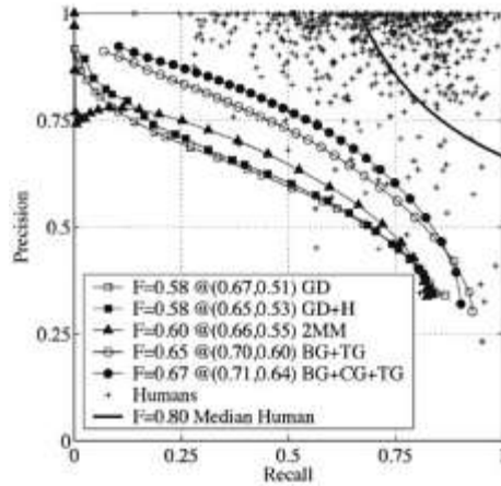
FIGURE 17.12: Martin et al. (2004) evaluate P_b (or probability of boundary) detectors by comparison to boundaries marked by humans. One plots the recall and precision of a set of boundaries for a given detector threshold by placing predicted points in correspondence with boundary points predicted by humans, weighting correspondences so that distant pairings are discouraged. Some predicted points are then unmatched, and so are false positives. Unmatched human boundary points give a count of false negatives. Varying the threshold gives a recall-precision curve. On this plot, the + signs are human informants, who differ from one another in where they place boundary points. The median F measure for humans is 0.8, and the human curve is the F = 0.8 curve. Using different subsets of the feature set gives slightly different performance statistics; using all the features we have described gives the BG + CG + TG curve. This figure was originally published as Figure 3 of “Learning to Detect Natural Image Boundaries Using Local Brightness, Color, and Texture Cues,” by D.R. Martin, C.C. Fowlkes, and J. Malik, IEEE Transactions on Pattern Analysis and Machine Intelligence, 2004 © IEEE 2004.
