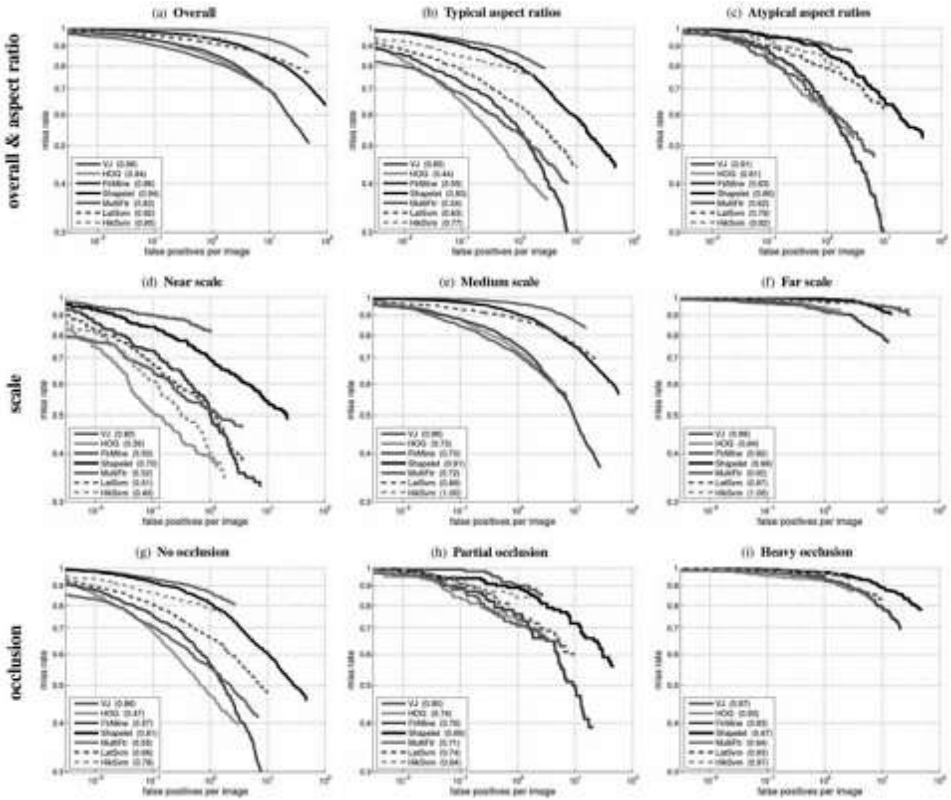
FIGURE 17.16: Performance of various pedestrian detectors for a test dataset ( top left , labeled “overall”) and for various special subsets of that test dataset, performed using the testbed of Dollar et al. (2009). Detectors that do well for some cases (for example, near-scale pedestrians) can do poorly for other cases (for example, medium-scale pedestrians). Some cases are hard for all detectors. This figure was originally published as Figure 9 of “Pedestrian Detection: A Benchmark” P. Dollár, C. Wojek, B. Schiele, and P. Perona, Proc. IEEE CVPR 2009 © IEEE 2009.
