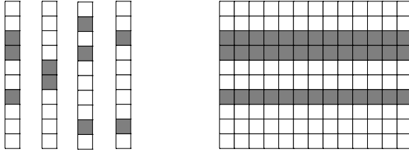
FIGURE 6.16: Sparsity vs. joint sparsity: Gray squares represents nonzero values in vectors (left) or matrix (right). Reprinted from “Non-local Sparse Models for Image Restoration,” by J. Mairal, F. Bach, J. Ponce, G. Sapiro, and A. Zisserman, Proc. International Conference on Computer Vision , (2009). © 2009, IEEE.
