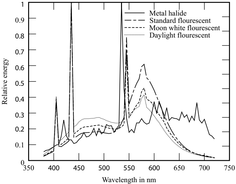
FIGURE 3.5: The relative spectral power distribution of four different lamps from the Mitsubishi Electric Corporation. Note the bright, narrow bands that come from the fluorescent phosphors in the fluorescent lamp. The figure was plotted from data made available by the Coloring Info Pages at http://www.colorpro.com/info/data/lamps.html ; the data was measured by Hiroaki Sugiura.
