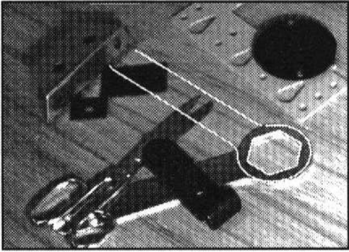
FIGURE 12.7: Edge orientation can be a deceptive cue for verification, as this figure illustrates. The edge points marked on the image come from a model of a spanner, recognized and verified with 52% of its outline points matching image edge points with corresponding orientations. Unfortunately, the image edge points come from the oriented texture on the table, not from an instance of the spanner. As the text suggests, this difficulty could be avoided with a much better description of the spanner's interior as untextured, which would be a poor match to the oriented texture of the table. This figure was originally published as Figure 4 of "Efficient model library access by projectively invariant indexing functions," by C.A. Rothwell et al., Proc. IEEE CVPR, 1992, © IEEE, 1992.
