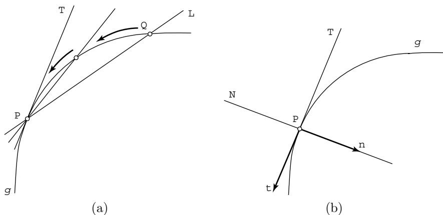
FIGURE 13.4: Tangents and normals: (a) definition of the tangent as the limit of secants, (b) the coordinate system defined by the (oriented) tangent and normal.
