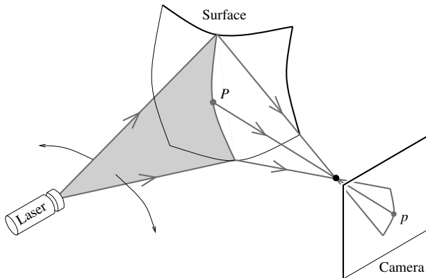
FIGURE 14.1: A range sensor using a plane of light to scan the surface of an object.
