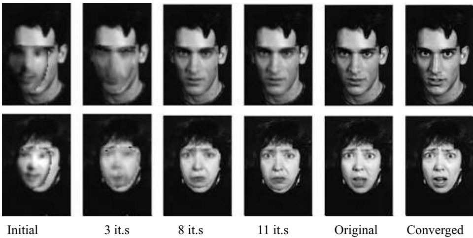
FIGURE 12.10: Active appearance models registered to face images. On the left , the initial configuration of the model (blurry blob over the face; original face is second from right). As the minimization process proceeds, the search improves the registration to produce, in the final converged state, the registration on the right . Once we have this registration, the location of the vertices of the mesh and the deformation parameters encode the shape of the face. This figure was originally published as Figure 5 of “Active Appearance Models,” by T. Cootes, G. Edwards, and C. Taylor, IEEE Transactions on Pattern Analysis and Machine Intelligence, 2001, © IEEE, 2001.
