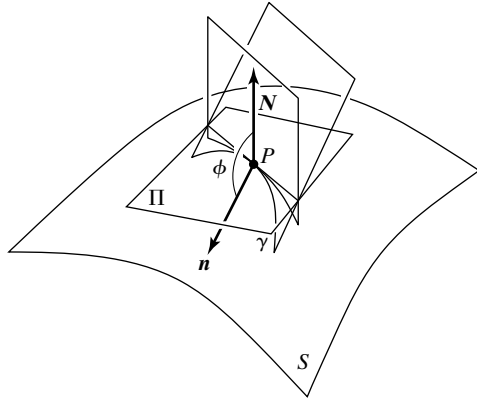
FIGURE 13.12: Meusnier's theorem.
