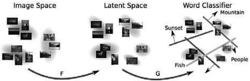
FIGURE 21.9: One way to build correlated linear classifiers is to learn a matrix of linear classifiers \mathcal{C} while penalizing the rank of \mathcal{C} . A low rank solution factors into two terms as \mathcal{C} = \mathcal{G}\mathcal{F} . The term \mathcal{F} maps image features to a reduced dimensional space of linear features, and \mathcal{G} maps these features to words. The word predictors must be correlated, because the number of rows of \mathcal{G} is greater than the dimension of the reduced dimensional feature space. This figure was originally published as Figure 1 of “Scene Discovery by Matrix Factorization,” by N. Loeff and A. Farhadi, Proc. European Conference on Computer Vision. Springer Lecture Notes in Computer Science, Volume 5304, 2008 © Springer, 2008.
