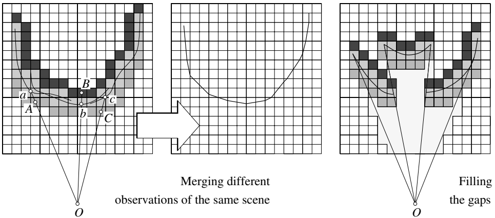
FIGURE 14.11: A 2D illustration of the Curless-Levoy method for fusing multiple range images. In the left part of the figure, three views observed by the same sensor located at the point O are merged by computing the zero set of a weighted average of the signed distances between voxel centers (e.g., points A , B , and C ) and surface points (e.g., a , b , and c ) along viewing rays. In general, distances to different sensors would be used instead. The light-gray area in the right part of the figure is the set of voxels marked as empty in the gap-filling part of the procedure.
