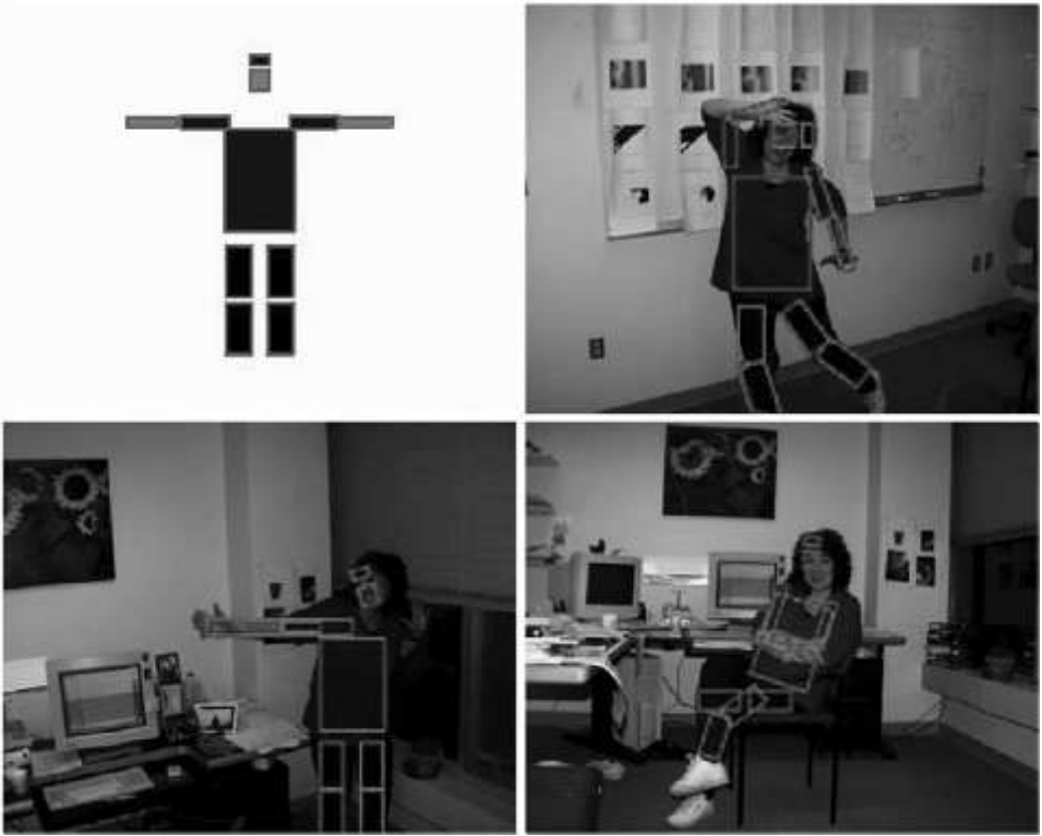
FIGURE 20.4: On the left , a tree-structured model of a person. Each segment is colored with the image color expected within this segment. The model attempts to find a configuration of these 11 body segments (nine limb segments, face, and hair) that (a) matches these colors and (b) is configured like a person. This can be done with dynamic programming, as described in the text. The other three frames show matches obtained using the method. This figure was originally published as Figure 4 of “Efficient Matching of Pictorial Structures,” by P. Felzenszwalb and D.P. Huttenlocher, Proc. IEEE CVPR 2000, © 2000, IEEE.
